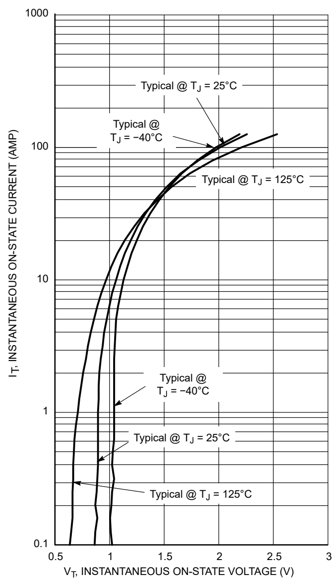
Figure 3. On-State Characteristics
