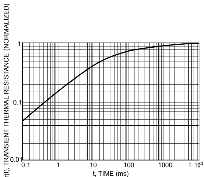
Figure 4. Thermal Response
