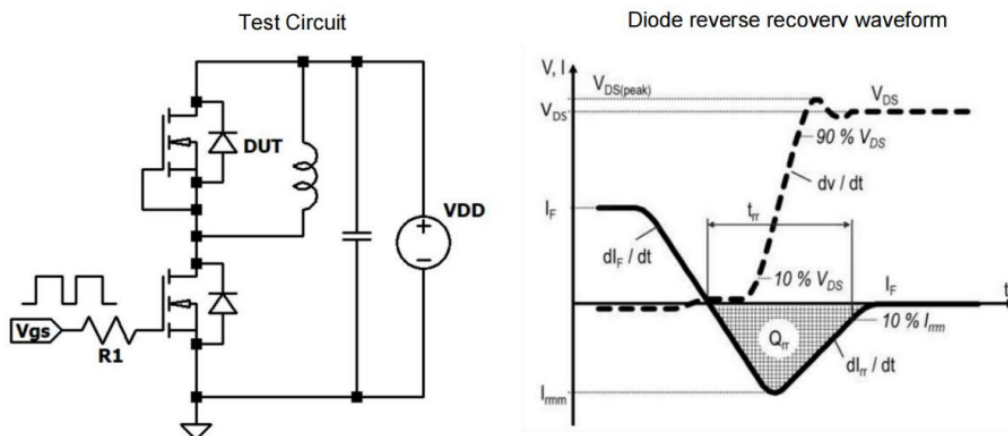
Fig B: Diode Recovery Test Circuit & Waveforms
