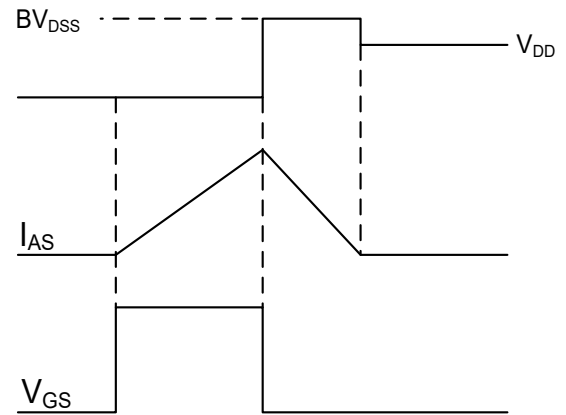
Fig.8 EAS Waveform
